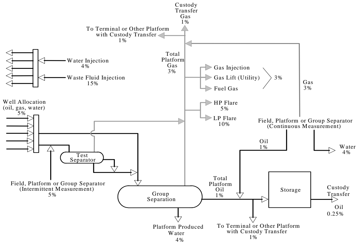
Figure 2 – Process Flow Diagram Showing Measurement Uncertainties
