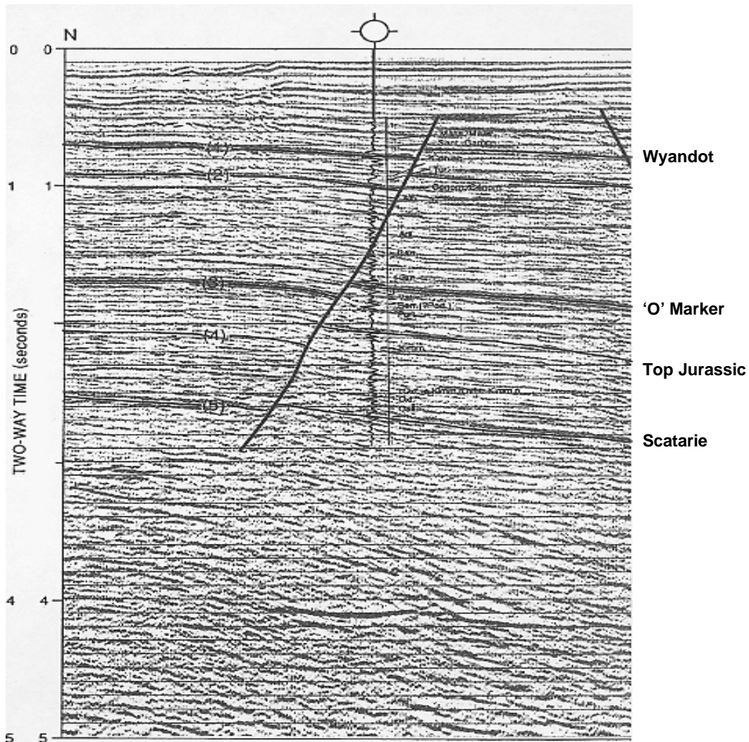
Figure 124. Seismic profile – Dover A-43 exploration well. See Figure 4 for location.
