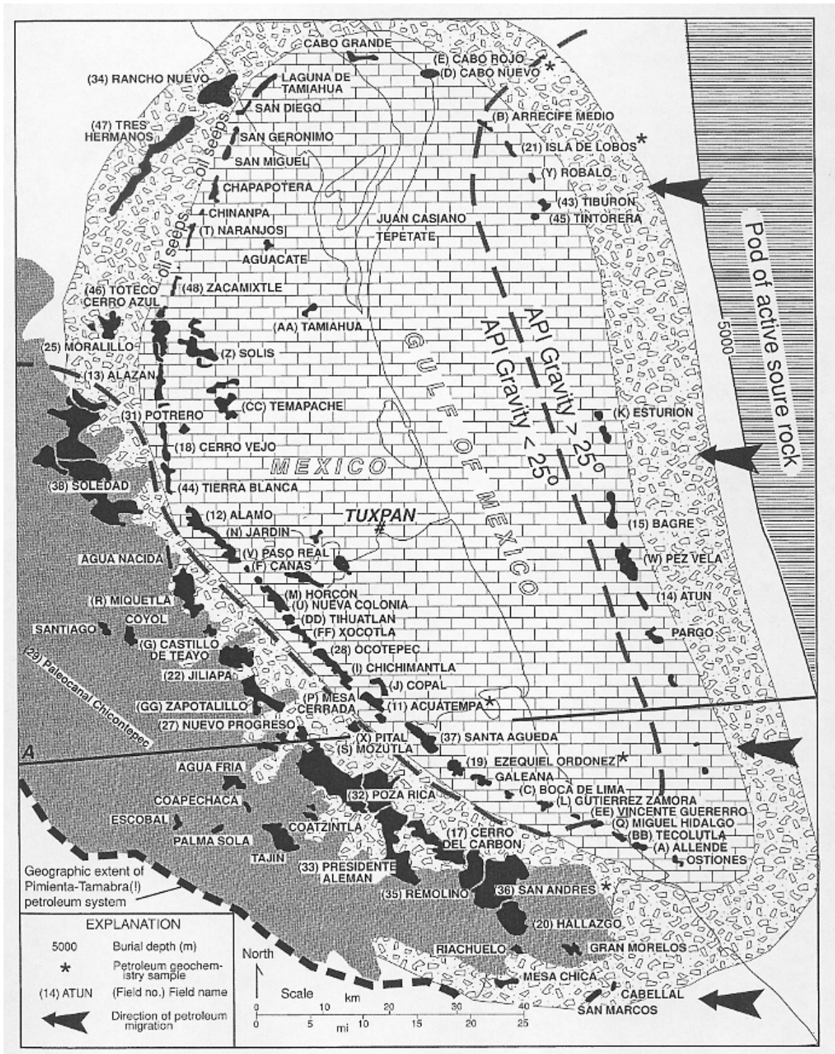
Figure 66. Map of Tuxpan area oil and gas fields (Magoon et al., 2001). Not the location of the source rock area and hydrocarbon migration pathways with the majority of fields in the margin-flanking debris flow breccias (USCG Assessment Units 2, 3, and 4).
