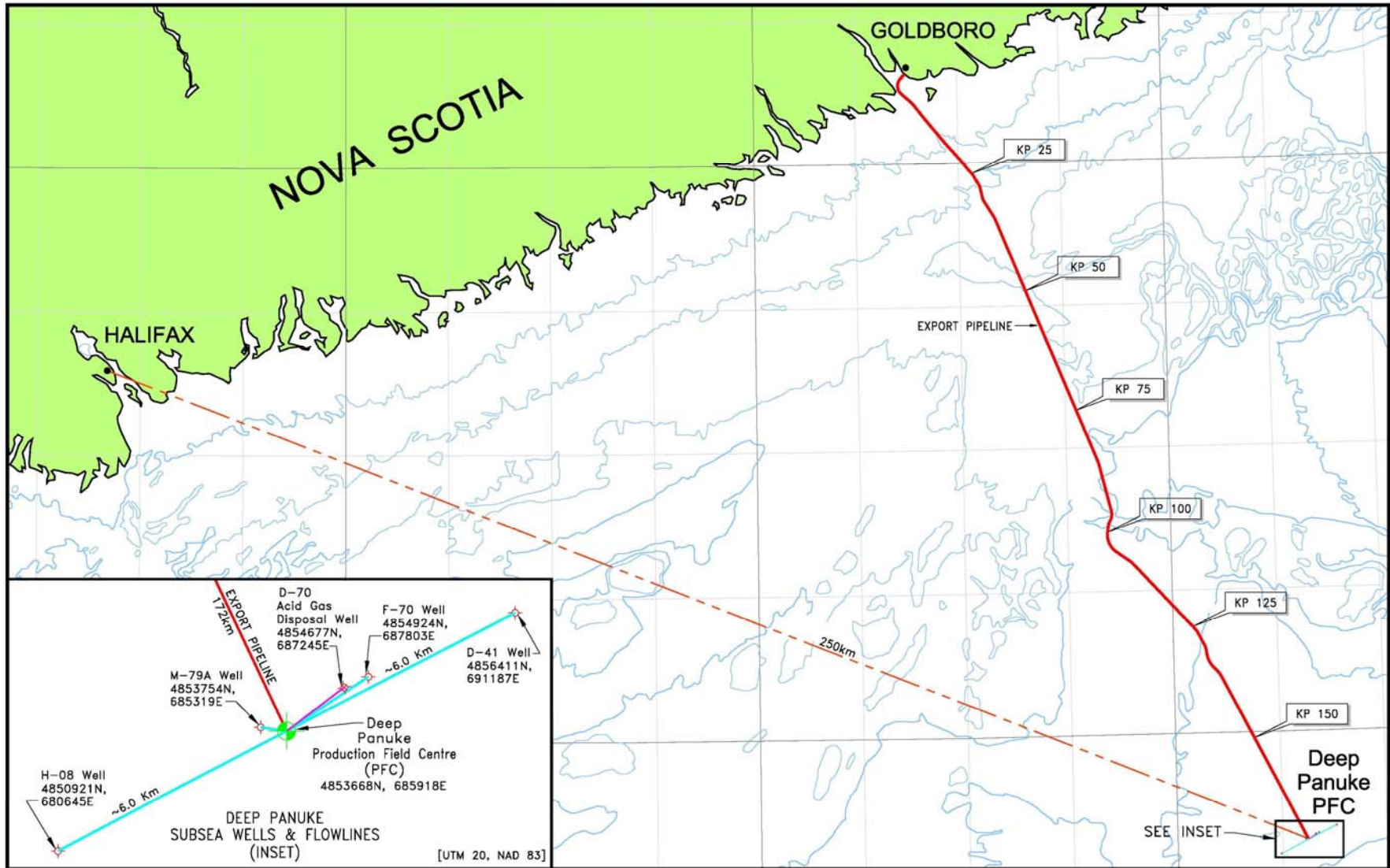
Figure 1.2 Offshore Pipeline Pre-Lay Survey Location Map
